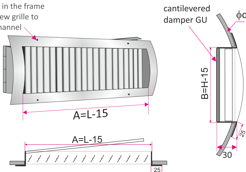
L, H - dimensions of the grille mounting hole
