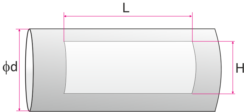
L, H - dimensions of the grille mounting hole
